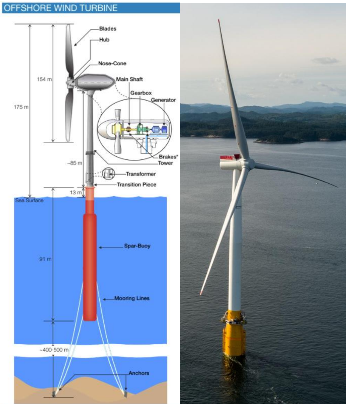
Figure 9. Original design of representative wind turbine, substructure, and mooring/anchoring system adapted from the Hywind Scotland commercial pilot park to deployment in federal waters off CA. 40
