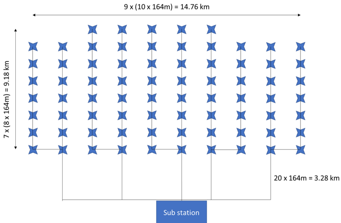
Figure 14. Example cable array.
