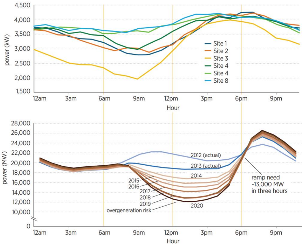
Figure 4. The “duck curve” and modeled generation profiles for 6-Mw offshore wind turbines at six California sites. Adding offshore wind into California’s electricity portfolio may help alleviate overgeneration and ramping challenges as solar and land-based wind generation continue to grow. 16
