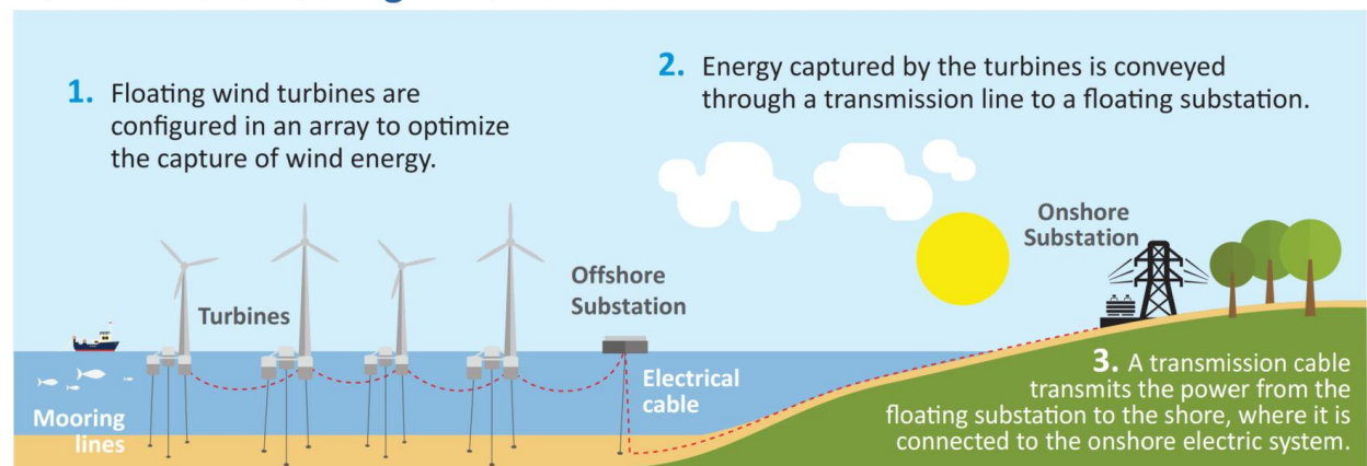
Figure 2. A general overview of a floating offshore wind farm. The wind turbines are connected to the ocean floor with mooring lines and an anchoring system. Then electric array cables connect the turbines to an offshore substation which then transmits the energy to the onshore grid. 5
