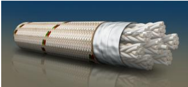
Figure 11. Manufactured by Lankhorst Offshore, GAMA 98 polyester ropes are made from high efficiency subrope cores laid parallel within an outer braided jacket. Each rope typically include 7 to 18 sub-ropes that result in a torque-free mooring line. 48
