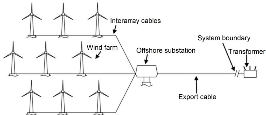
Figure 7. System boundary for a representative floating offshore wind project, adapted from Thomson and Harrison, 2015. 28
