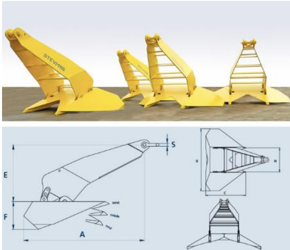
Figure 12. Anchor geometry provides an extremely high weight/strength ratio. The fluke shape minimizes soil disturbance during penetration and its enlarged surface provides holding power. The fluke width provides stability both on the seabed and during penetration. 51
