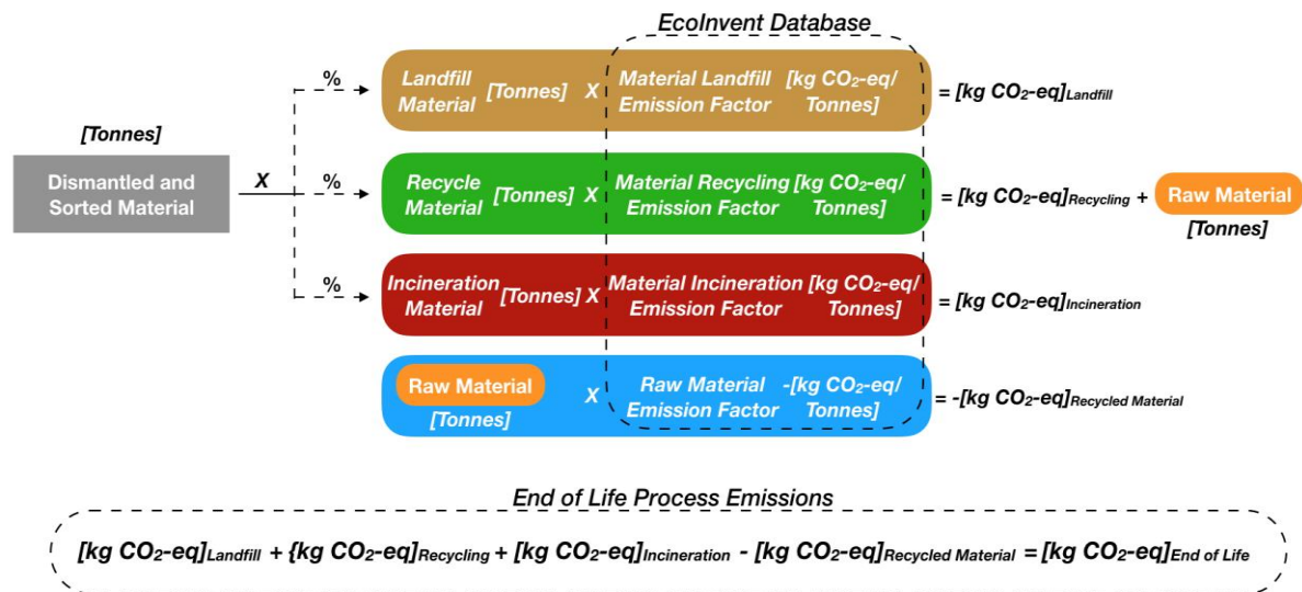
Figure 16. LCA Process Flow of End of Life (EOL) Treatment.
