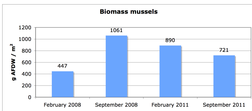
Figure 10. Average biomass (g AFDW per m 2 ) of common mussel ( Mytilus edulis ) in the collected samples on the monopiles in OWEZ.
