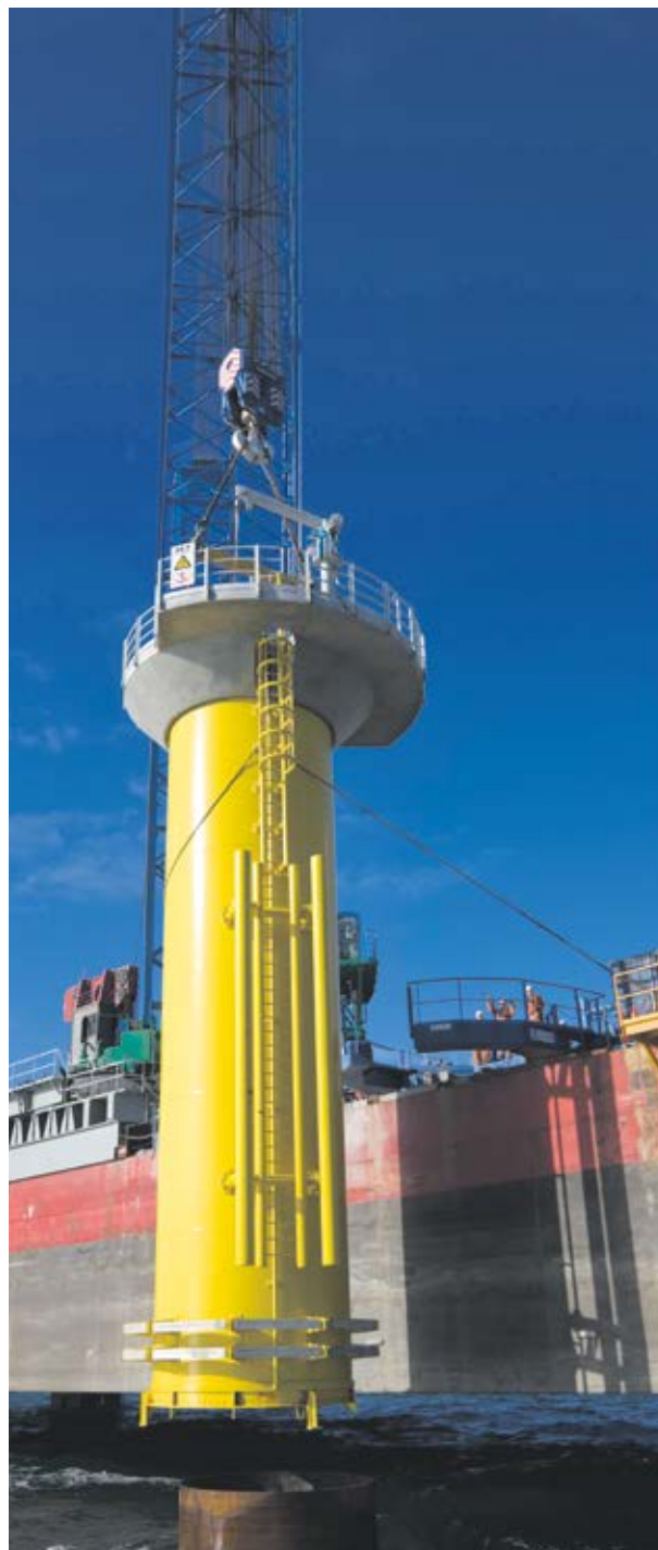
Preparation of monopile foundation at Horns Rev 2.
