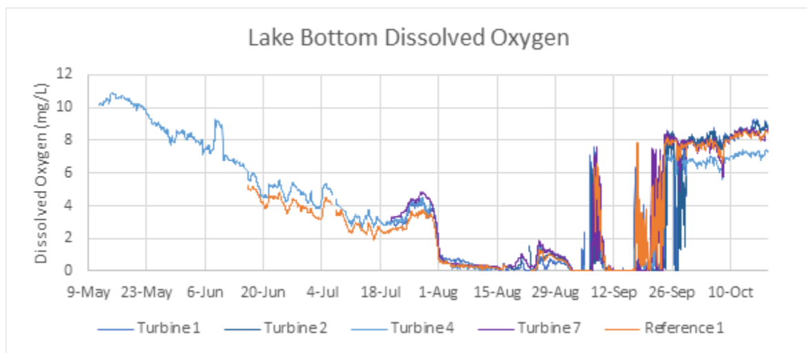
Figure 12. 2016 lake bottom dissolved oxygen at Turbine sites 1, 2, 3, 7, and Reference 1.
