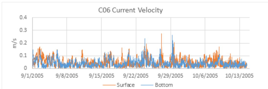
Figure 14. 2005 IFYLE current velocity from the lake surface and bottom at station C06.
