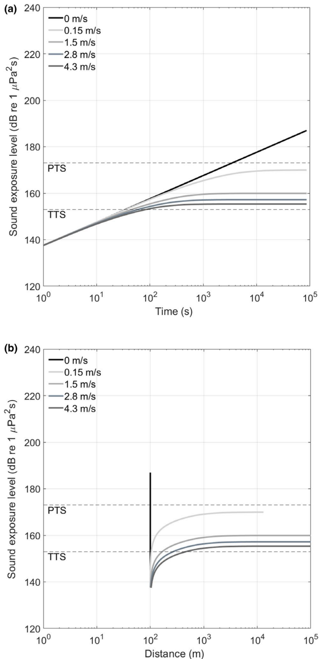
FIGURE 6 Very high-frequency cetacean weighted sound exposure levels ( SEL_w ; dB re 1 \mu Pa^2 s ) for stationary and fleeing harbour porpoise accumulated at 1-s intervals up to 24 hr. Figure indicates SEL_w over (a) time (s) and (b) distance (m) assuming the animal is at 100 m from an Airmar acoustic deterrent device (ADD) at its onset. Dashed lines indicate temporary threshold shift (TTS) or permanent threshold shift (PTS)
