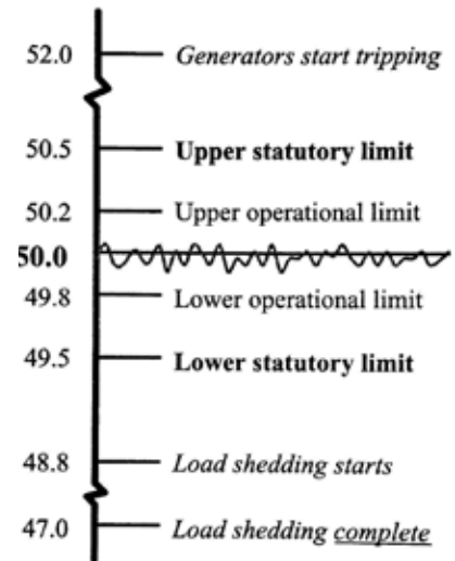
Figure 3-7: Frequency Range in hz (Freris & Infield, 2008)
