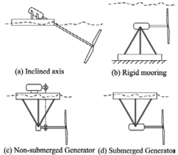
Figure 3-2: Horizontal Axis Turbines (Kahn et al. 2009)
