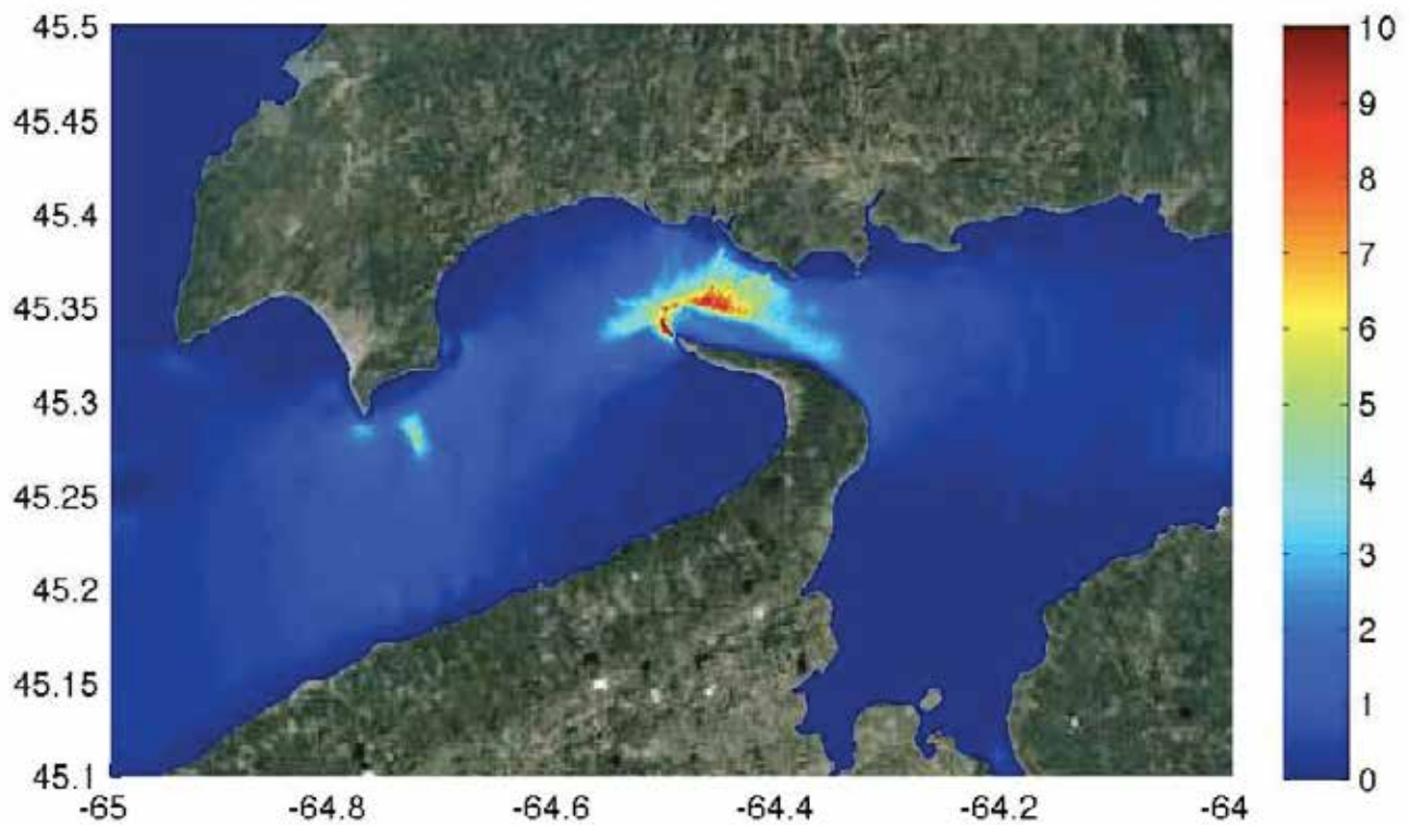
Figure 2-5: Mean Power Density in kW/m² for Minas Channel
