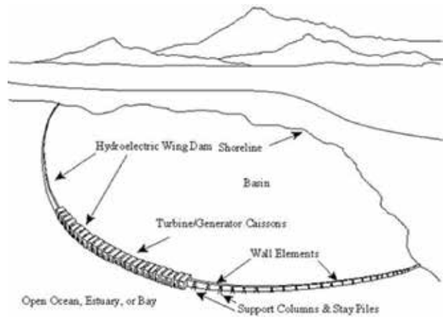
Figure 1-7: Diagram of a Shore-attached Tidal Impoundment.
