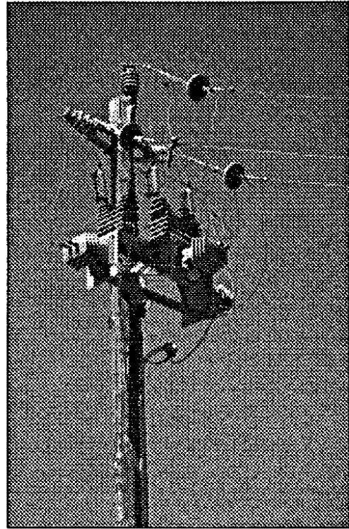
Metering pole
