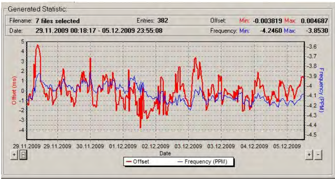
Figure 6-107. Plot of the time offset between the SEAAR2l radar DRP at SEA and the United States NTP time pool.
