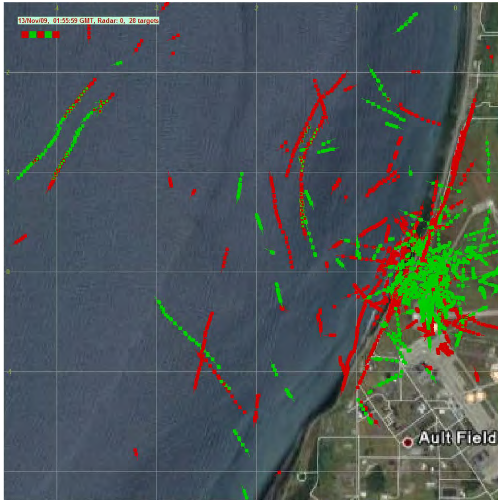
Figure 6-108: COP display showing fused tracks from the WIAR1 and eBirdRad radars at NAS Whidbey Island on 13 November 2009 at 01:55 UTC. Red tracks = WIAR1 radar; green tracks = WIEBirdRad radar.
