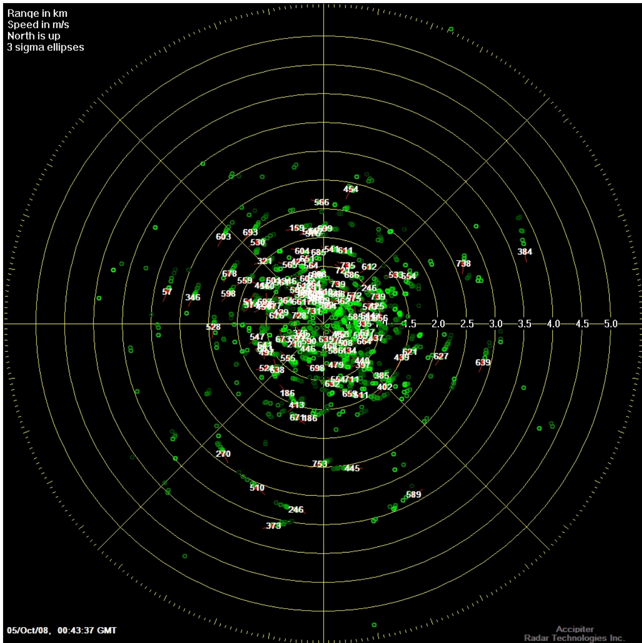
Figure 6-57. Digital image of the display of the eBirdRad radar at Edisto Island, South Carolina on 5 October 2008 GMT. The radar was equipped with a dish antenna that had a 2.5° beam width and was inclined 30° above horizontal. The range rings in the display are in kilometers. The green circles are detections; the red squares with white numbers (Track ID) indicate the current position of a tracked target.
