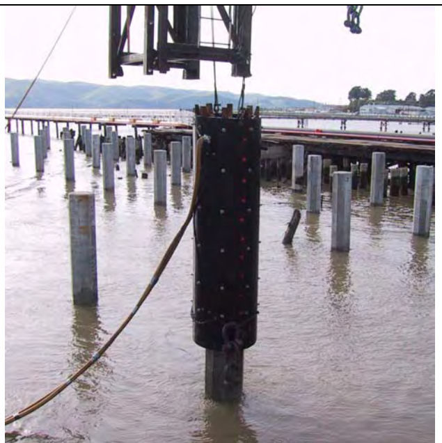
Figure I.5-4b “Bubbleator” Used to Attenuate Underwater Sound
