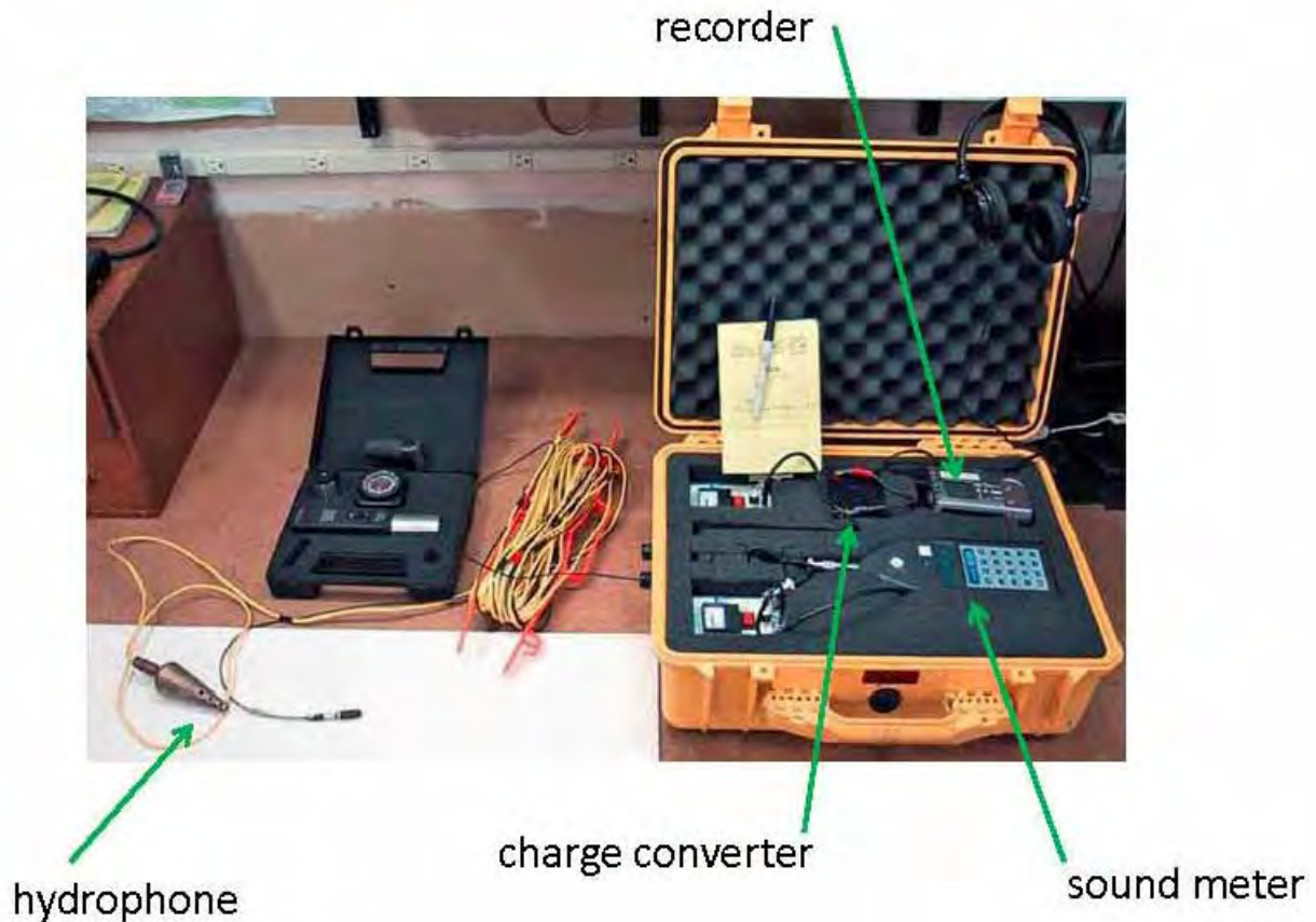
Figure 2-16. Measurement System
