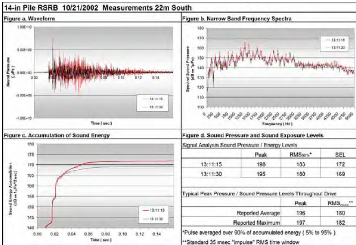
Figure I.10-3 Representative Signal Analyses for 14-Inch-Diameter Pile. Pulse received at 22 meters from the pile at Richmond-San Rafael Bridge.
