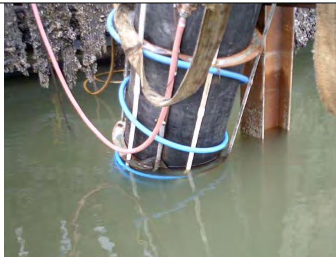
Figure I.4-2b Close-View of Confined Air Bubble Attenuation System next to Vertical H-Type Pile
