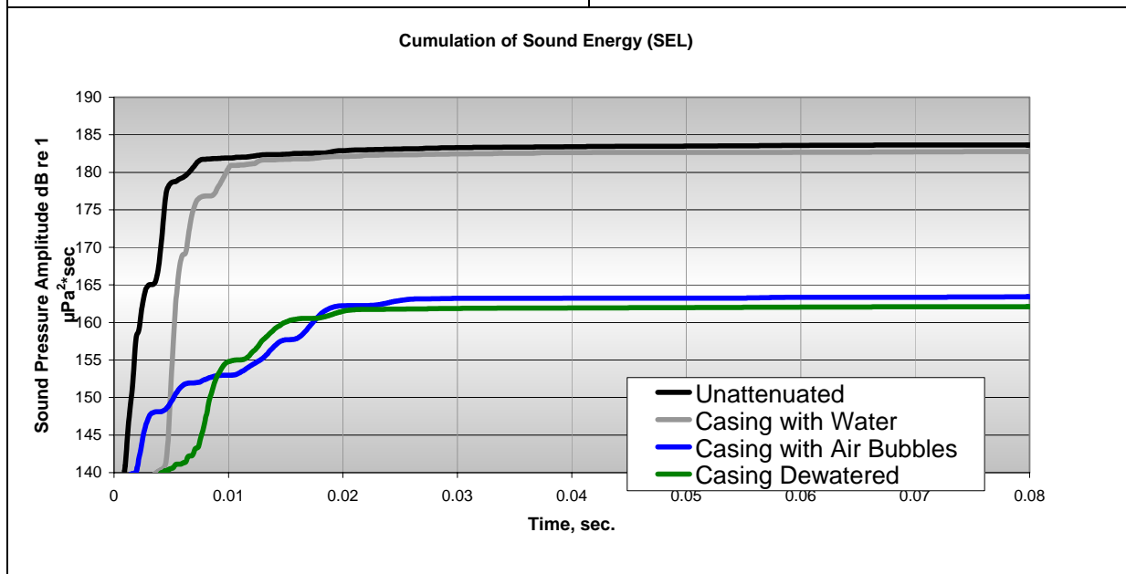
Figure I.8-5 Signal Analyses of Underwater Sound Pulses at 54 Meters – Isolation Casing Tests
