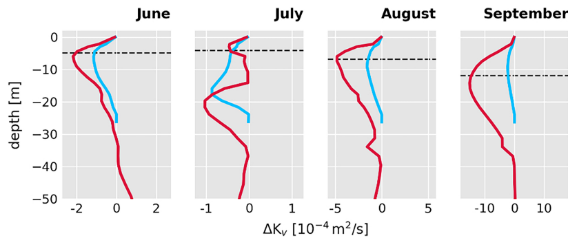
FIGURE 10 | Monthly mean profiles in mixing rate for the period of June to September. The dashed lines indicate the location of the mixed layer depth. For the profiles, grid points within 5 km around each wind farm were considered. Profiles are divided into deep ( z \geq 25 m, red lines) and shallow ( z < 25 m, blue lines) water depths.
