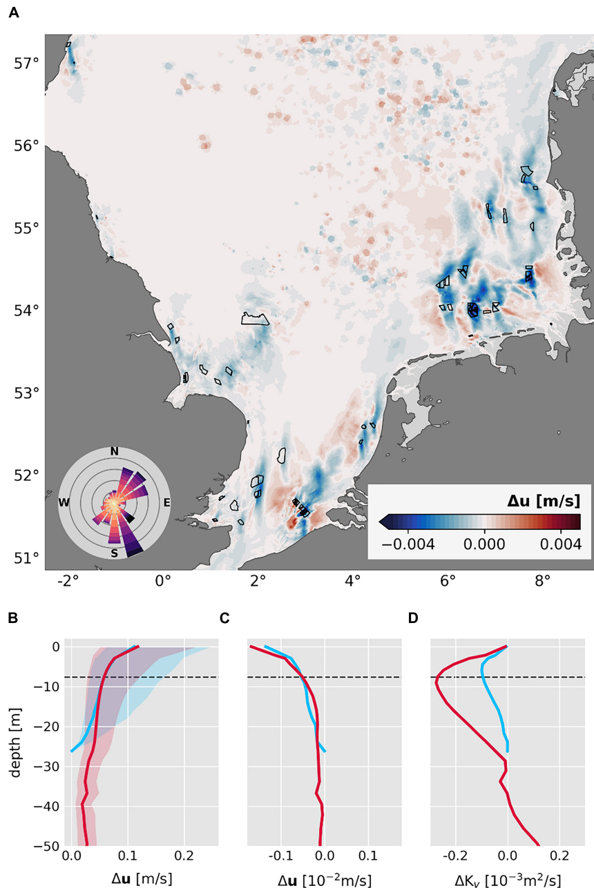
FIGURE 6 | Mean changes in horizontal velocity ( u ) and mixing rate ( K_v ). (A) Mean changes in horizontal sea surface velocity for daily mean data in the month of May. Black polygons indicate offshore wind farms. The wind rose indicates the direction in which the wind blew (color range between 1 and 12 m/s). Mean vertical profiles for the mean horizontal velocity (B) , the mean changes in horizontal velocity (C) , and the mean changes in mixing rate (D) at wind farms for the month of May 2013. Filled envelopes in panel (B) demonstrate the temporal variability during May. Dashed lines indicate location of the mixed layer depth. For the profiles, grid points within 5 km around each wind farm were considered. Profiles are divided into deep ( z \geq 25 m, red lines) and shallow ( z < 25 m, blue lines) water depths.
