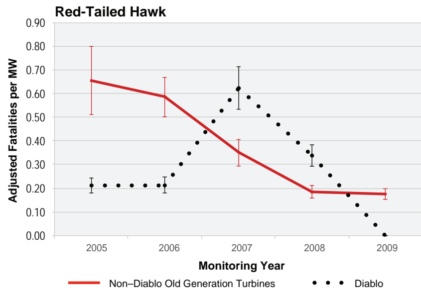
Figure 3-9 Comparison of Annual Adjusted Fatality Rates (Fatalities per MW ± 95% CI) at Diablo Winds and Non-Diablo Winds Older-Generation Turbines for the Four Focal Species in the APWRA, Monitoring Years 2005–2009
