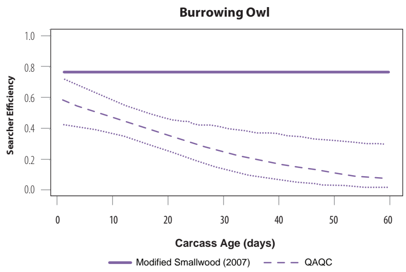
Figure C-3 Changes in Searcher Efficiency (and 95% Credible Interval Bands) as Carcasses Age Based on Blind Searches Conducted during the QAQC Study for the Four Focal Species in the APWRA
