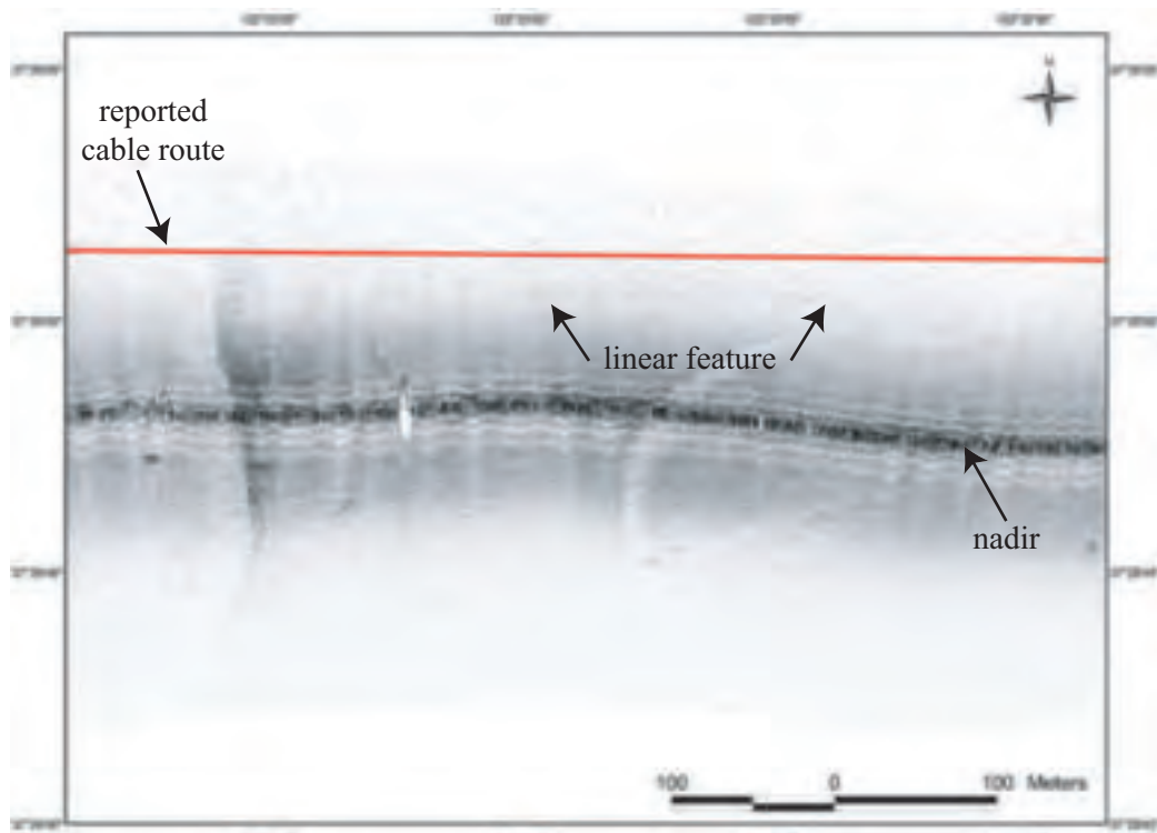
Figure 6: Side scan sonar image showing a linear reflection. Red line is the reported path of the ATOC/Pioneer Seamount cable (Appendix C). The nadir is an artifact. Linear feature extends from 37°29'50"N, 122°33'04"W to 37°29'51"N, 122°32'53"W.
