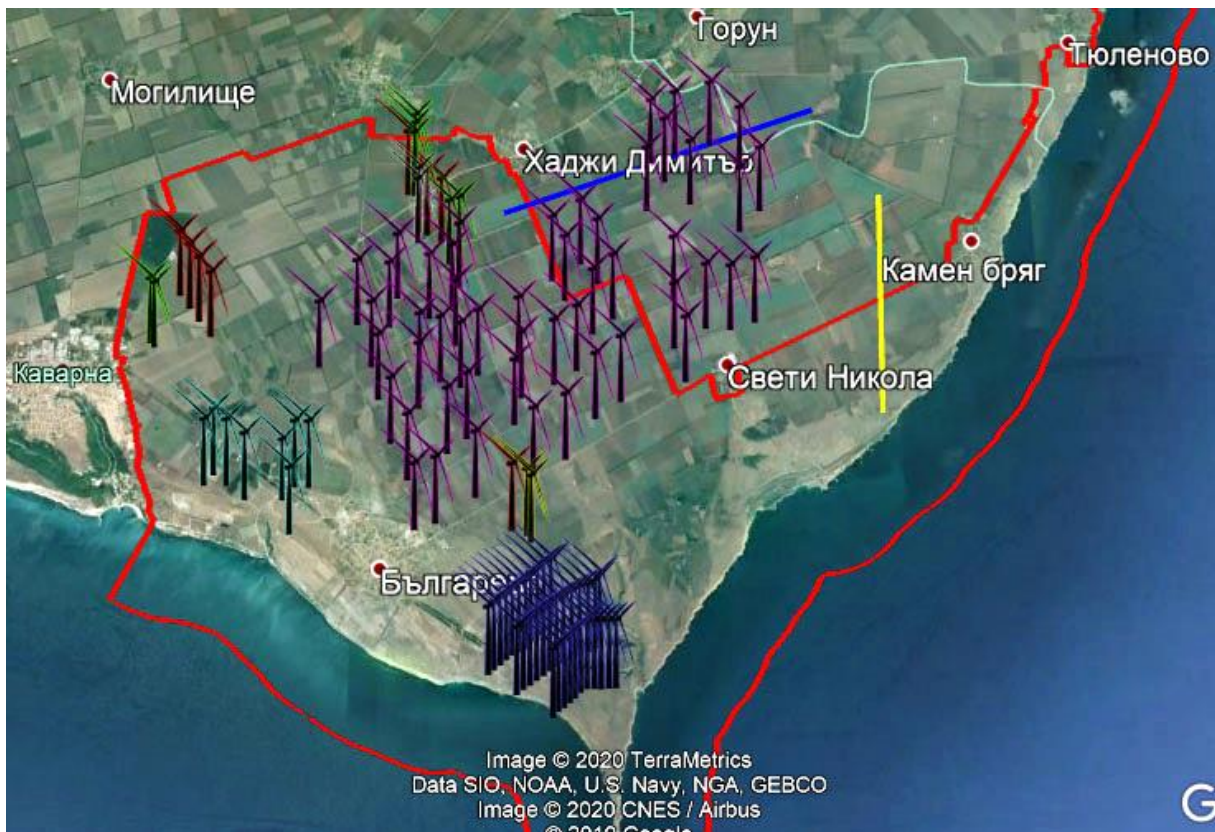
Figure 7. A flock of GWFG A. albifrons (blue) and C. cygnus (yellow) observed on 01 February 2020.
