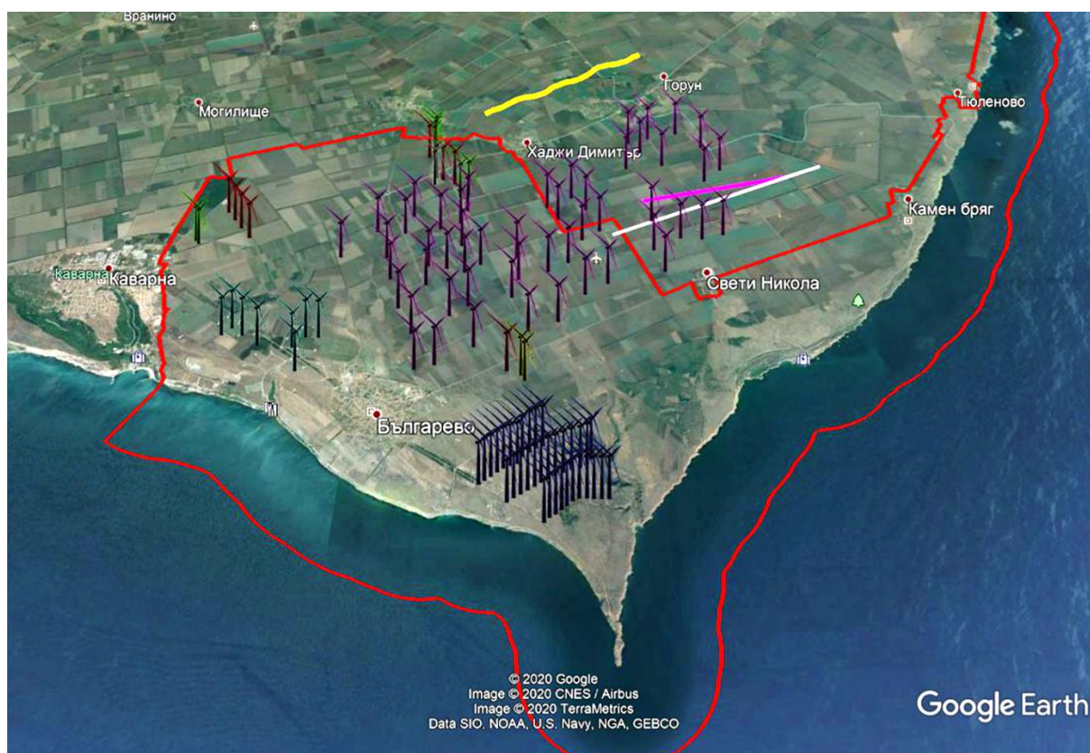
Figure 9. Flocks of 12 C. cygnus (white) observed on 13 February, 55 B. ruficollis (pink) observed on 12 February and 57 mixed geese (yellow) observed on 15 February 2020.
