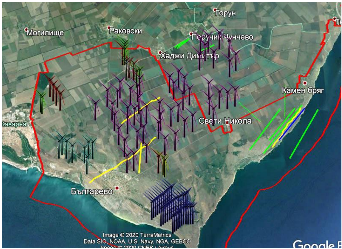
Figure 6. Flocks of GWFG A. albifrons (green), GG A. anser (blue) and mixed geese (yellow) observed in January 2020
