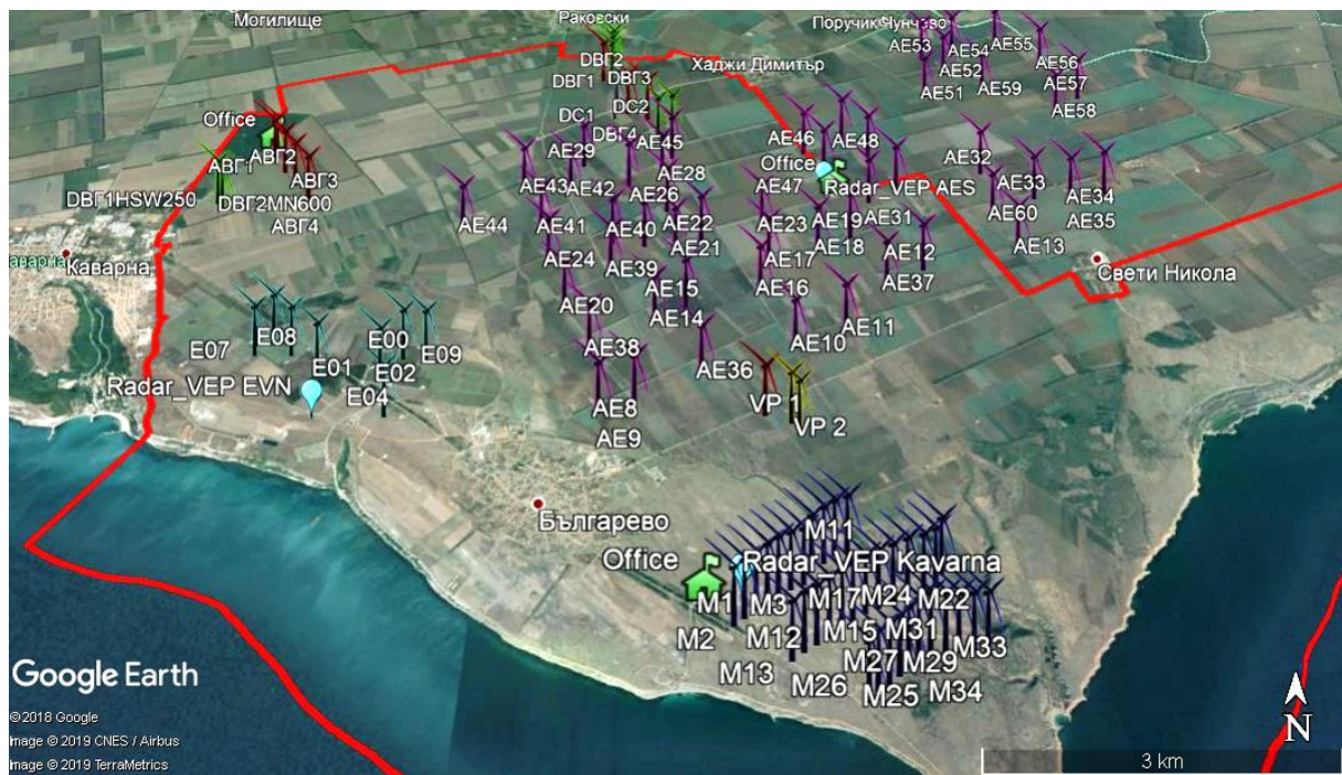
Figure 10. Locations of turbines searched for collision victims according to the codes given in Table 2
