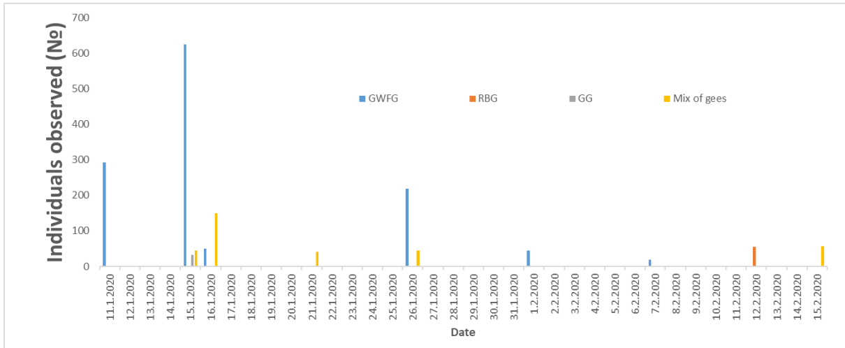
Figure 3. Temporal dynamics of wintering geese observed in ISPB territory during the winter season 2019-2020.
