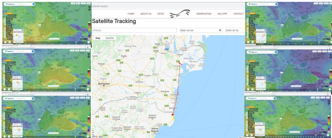
Figure 5. Ambient temperature and location of RBG with satellite transmitters in the days of February 2020 when the majority of geese were observed in ISPB territory ( https://www.ventusky.com/ and https://savebranta.org/en/birds-tracker )
