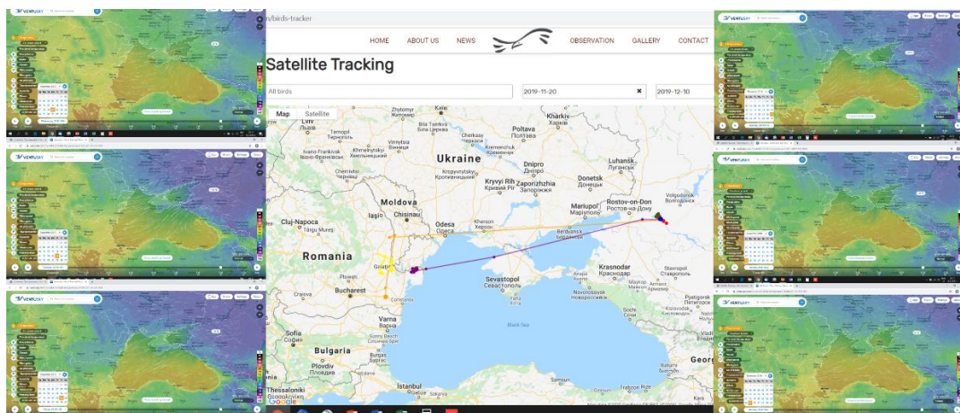
Figure 4. Ambient temperature and location of RBG with satellite transmitters in November, December 2019 according to web site information ( https://www.ventusky.com/ and https://savebranta.org/en/birds-tracker )
