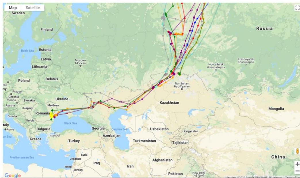
Figure 2 According to the Life program project website only one of over 10 RBG fitted with transmitters was registered in Bulgaria - in only one day during the winter of 2019-2020 ( https://savebranta.org/en/birds-tracker )
