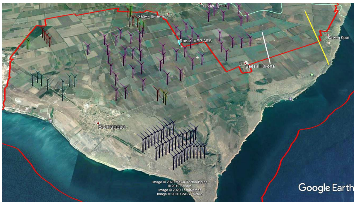
Figure 8. A flock of GWFG A. albifrons (white) observed on 07 February and C. cygnus (yellow) observed on 03 February 2020.
