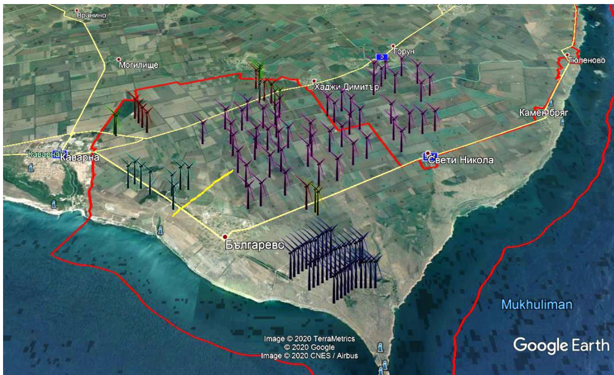
Figure 10. A flock of 12 C. Columbianus (yellow) observed on 19 February 2020.
